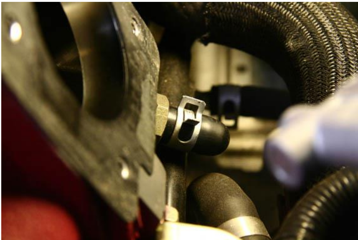
19. Remove the PCV valve and replace with 1/4" pipe plug.
